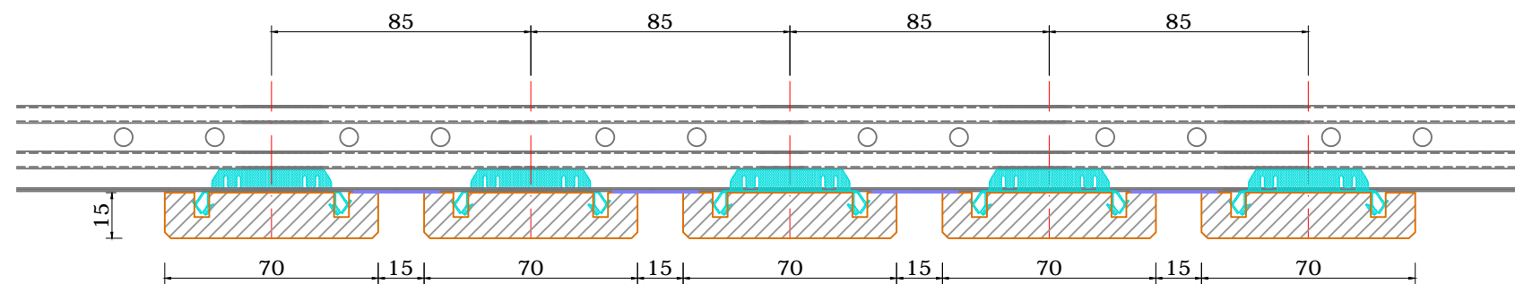
Cross section B-B
