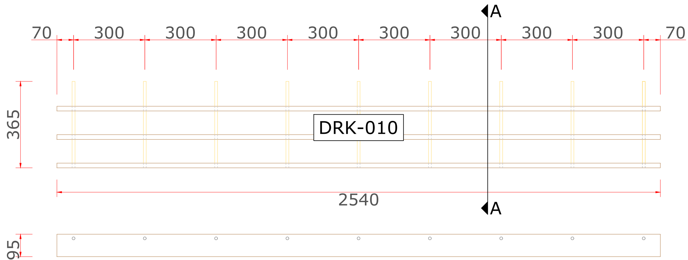
Front view
