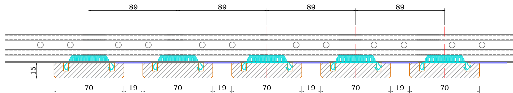
Cross section B-B
