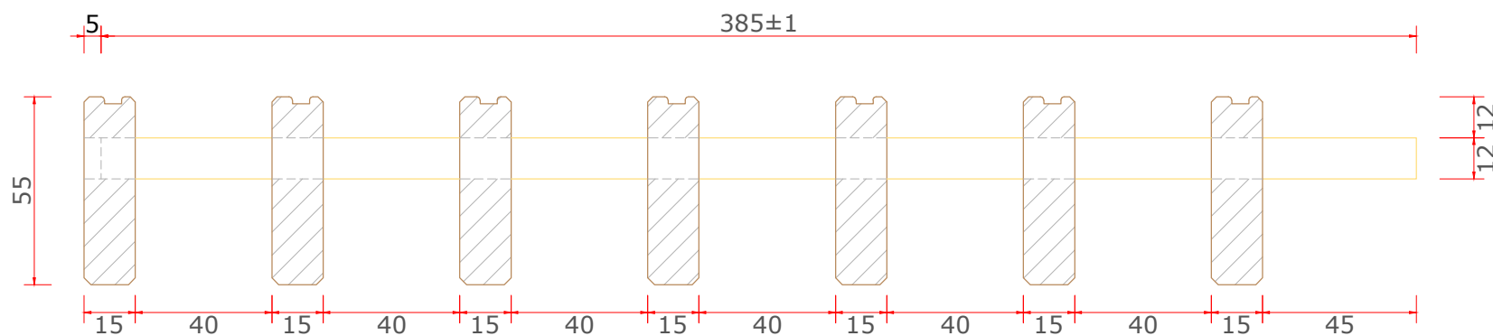
Cross section grill A-A
