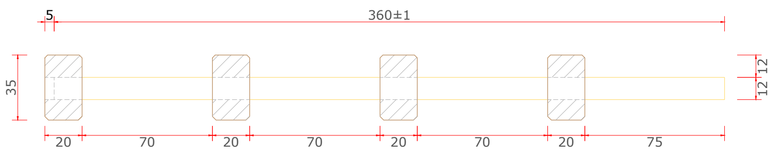
Cross section grill A-A
