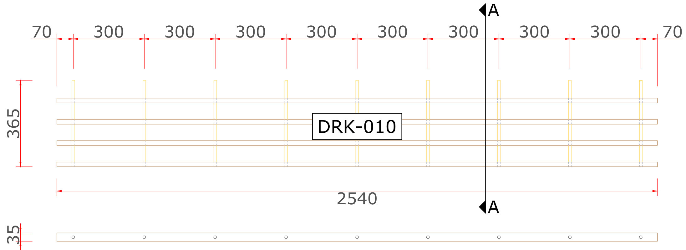
Front view
